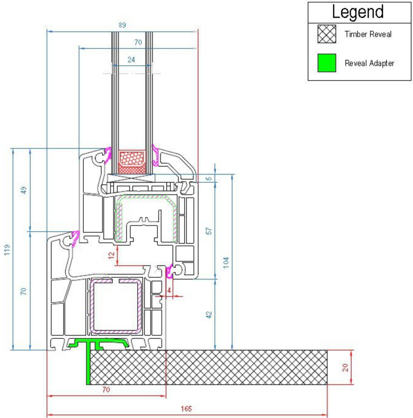
TIMBER REVEAL WITH REVEAL ADAPTER (FOR NEW CONSTRUCTION)
