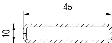
IFI 209121 s=1.5mm 3.0/0.2cm4 Reinforcements
