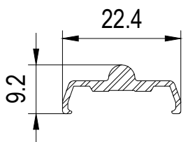
207120 Runner rail
