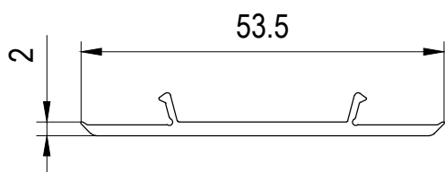
120293 Cover trim
