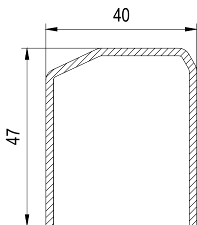
IFI 209192 s=1.25mm 4.6/3.7cm4 209193 s=2.0mm 7.0/5.7cm4 Reinforcements
