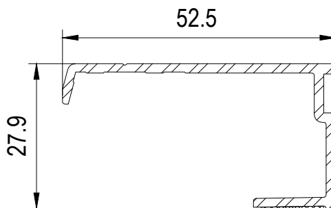
200122 Step protection Compatible brush seal: 459932 black
